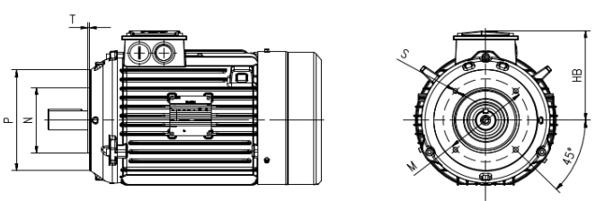
小凸缘安装型电机 IM3601, B14 Small flange-mounted motor IM3601, B14
